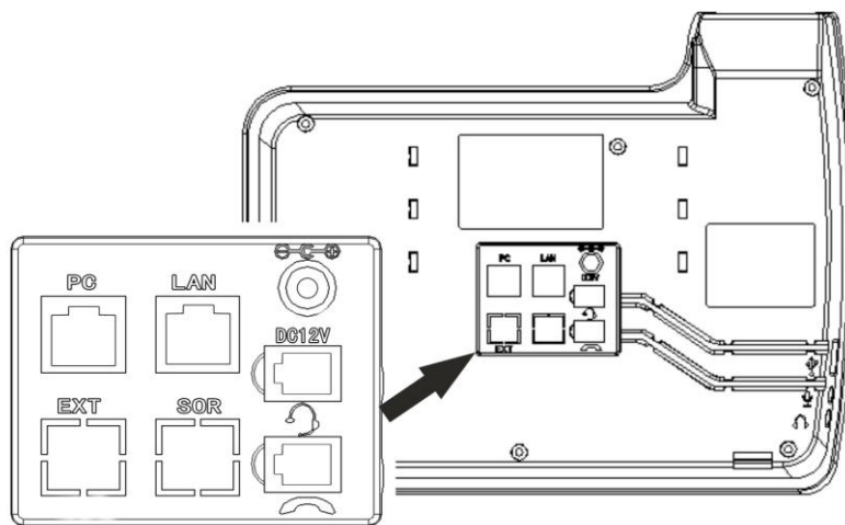
Figure 1 Connections on the back of IPitomy IP320
